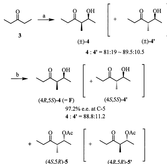
Scheme 4. Synthesis of 4
